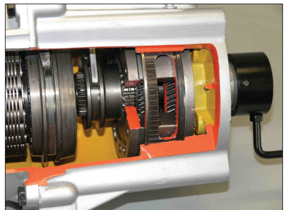
Transfer Case (High Range Position) Close-Up (model 1230)
